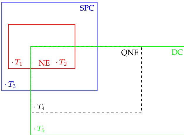
Figure 1. Diagram of the relationships between the classes NE , QNE , SPC and DC
